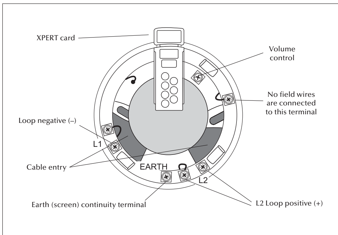
Ancillary base sounder—connection diagram
